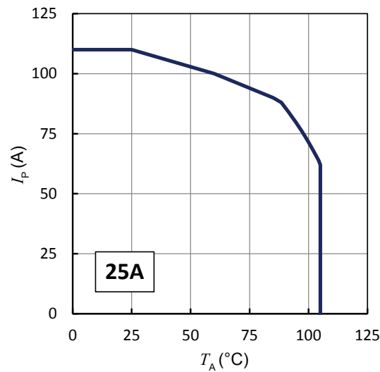
Figure 18: I_p vs T_A for HO series
