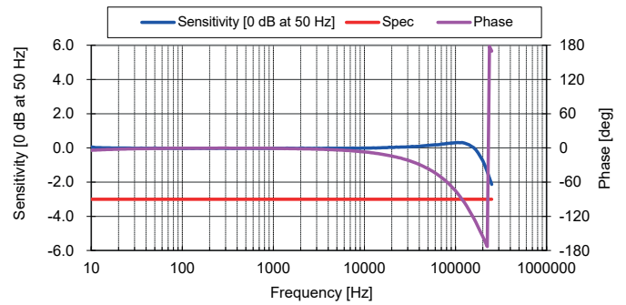
Figure 7: Frequency response
