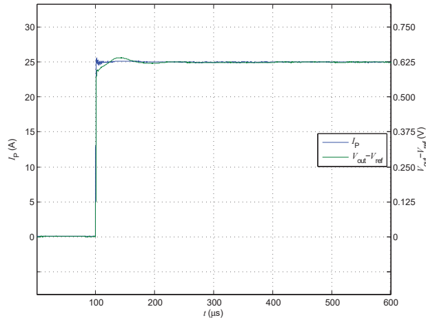
Figure 3: Step response
