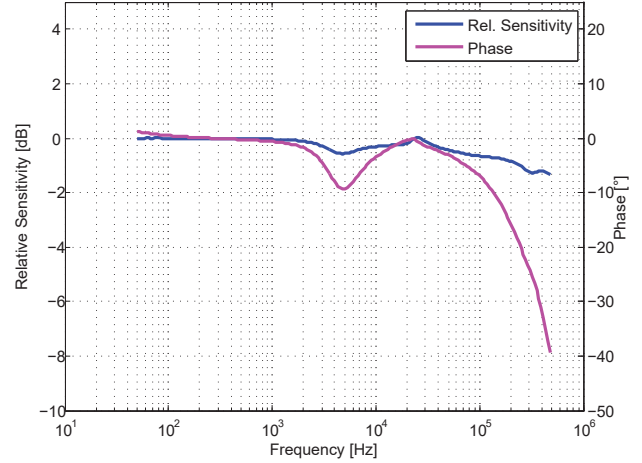
Figure 2: Frequency response
