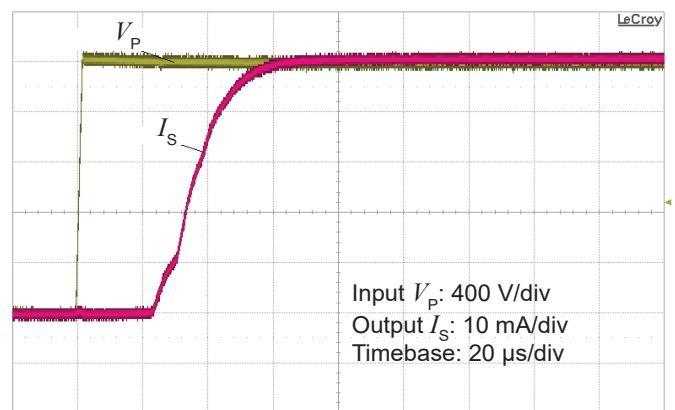
Figure 6: Typical step response (0 to 2000 V)
