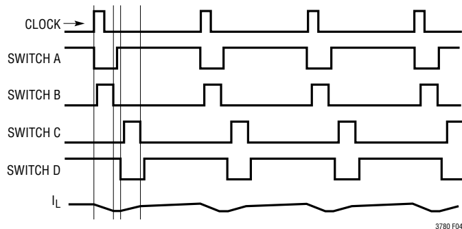
Figure 4a. Buck-Boost Mode ( V_{IN} \geq V_{OUT} )
