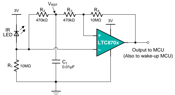
Figure 5. IR Receiver AFE Using LTC870x
