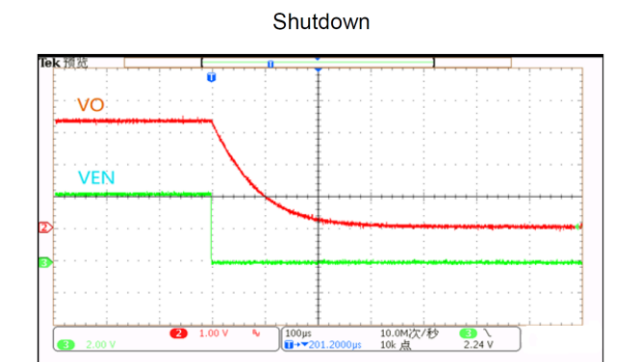
C_{IN}/C_{OUT} = 1\ \mu\text{F} , V_{EN} = 4.3\text{ V} , V_{OUT} = 3.3\text{ V} , I_{OUT} = 1\text{ mA}
