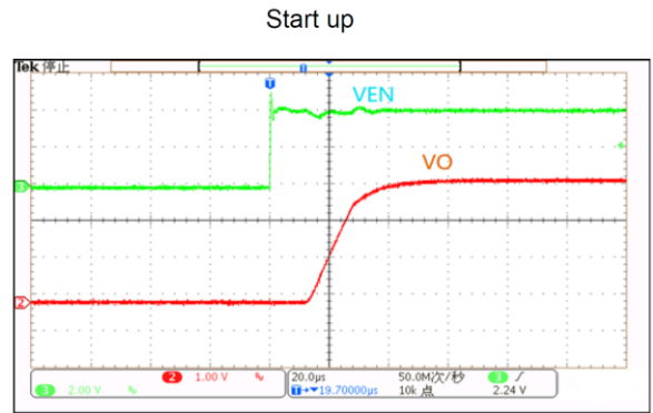
C_{IN}/C_{OUT} = 1\ \mu\text{F} , V_{EN} = 4.3\text{ V} , V_{OUT} = 3.3\text{ V} , I_{OUT} = 1\text{ mA}
