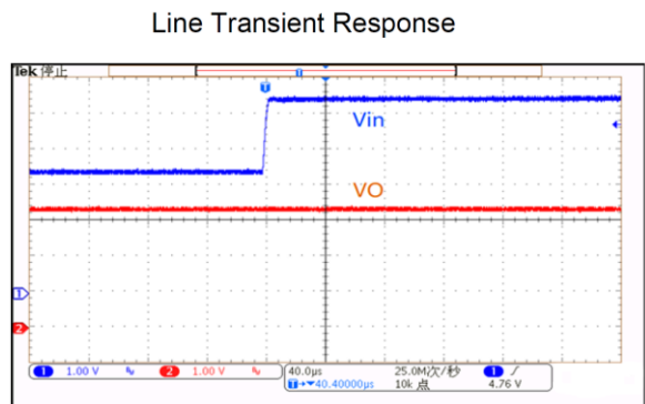
C_{IN}/C_{OUT} = 1\ \mu\text{F} , V_{IN} = 4\text{ V to } 6\text{ V} , V_{OUT} = 3.3\text{ V} , I_{OUT} = 1\text{ mA}
