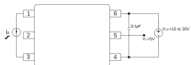
Figure 18 : I_{FH} Test Circuit
