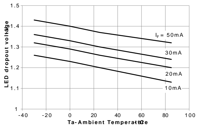
Fig 4. LED dropout voltage vs. Ambient Temperature
