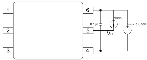
Figure 15 : V_{OL} Test Circuit
