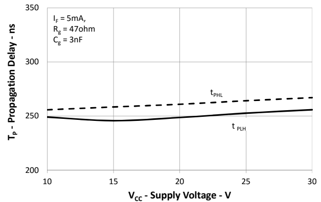
Figure 10. Propagation Delay vs. V_{cc}
