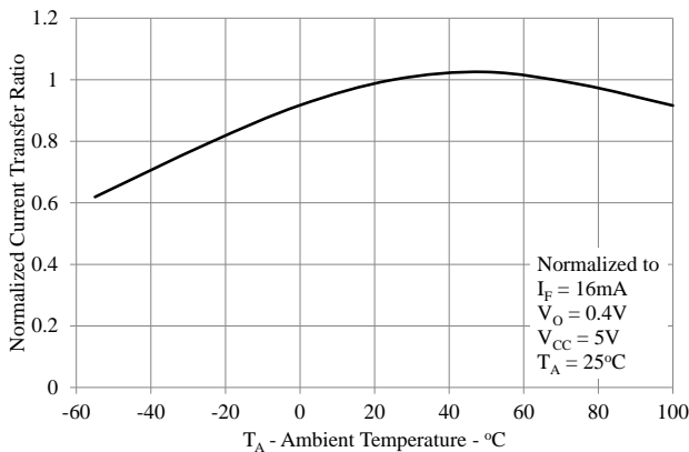
Figure 5: Current Transfer Ratio vs. Temperature.
