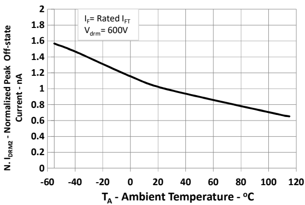
Fig.9 Normalized I_{DRM2} vs. T_A
