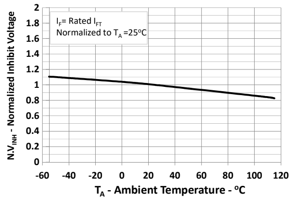
Fig.10 Normalized V_{INH} vs. T_A
