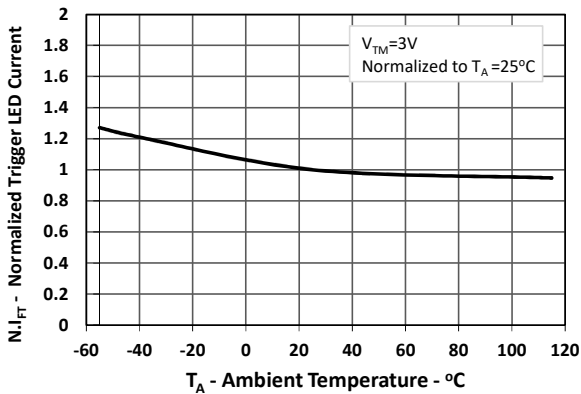
Fig 3. Normalized I_{FT} vs. T_A
