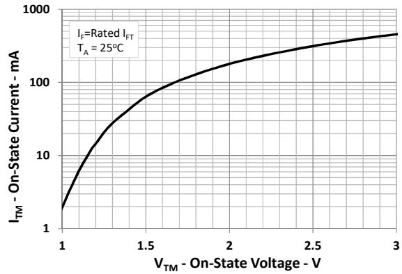
Fig.8 Normalized I_{TM} vs. V_{TM}
