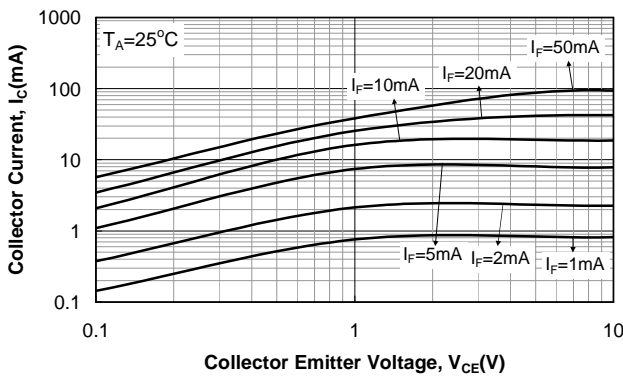
Figure 8. I_C vs. V_{CE}
