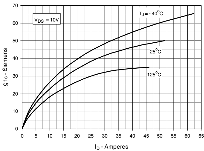
Fig. 9. Transconductance
