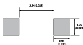
Mounting Pad Layout
