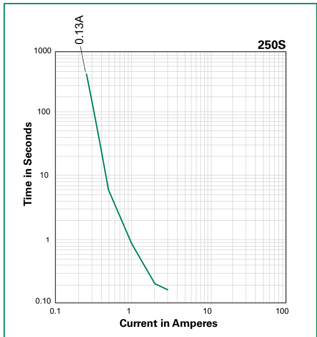
The average time current curves and Temperature Derating curve performance is affected by a number of variables, and these curves provided as guidance only. Customer must verify the performance in their application.
