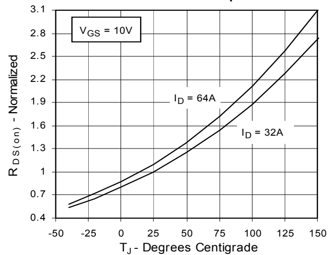
Fig. 4. R_{DS(on)} Normalized to I_D = 32A Value vs. Junction Temperature
