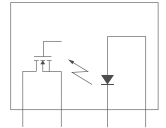
1-Form-A Unidirectional
