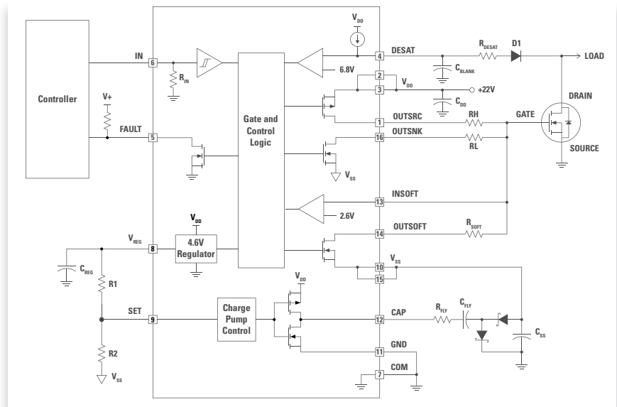
Typical IX4351 Application Circuit
