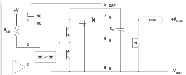
CPC1590 Application Diagram
