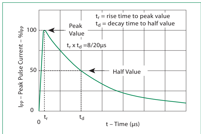
Figure 2 - Pulse Waveform
