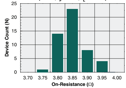
Typical On-Resistance Distribution (N=50, I_F=0mA , I_L=75mA )
