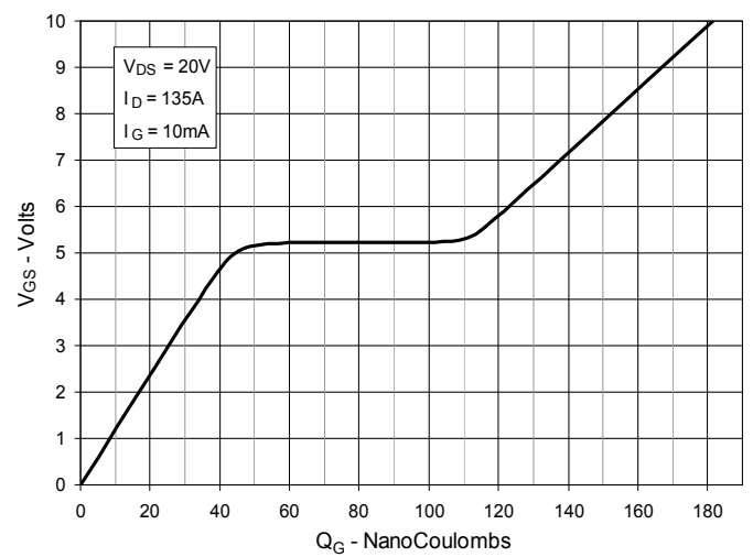
Fig. 10. Gate Charge
