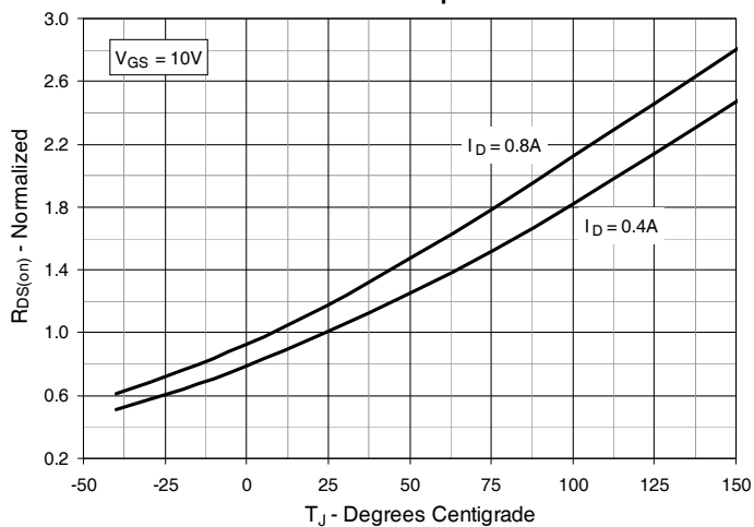
Fig. 4. R_{DS(on)} Normalized to I_D = 0.4A Value vs. Junction Temperature
