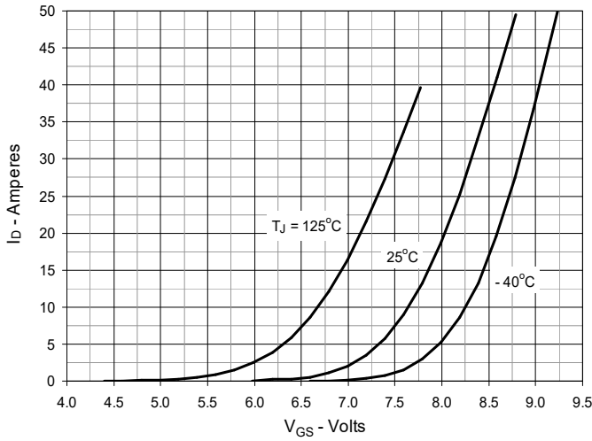
Fig. 7. Input Admittance
