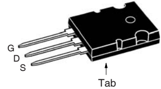
TO-264 (IXFK)
