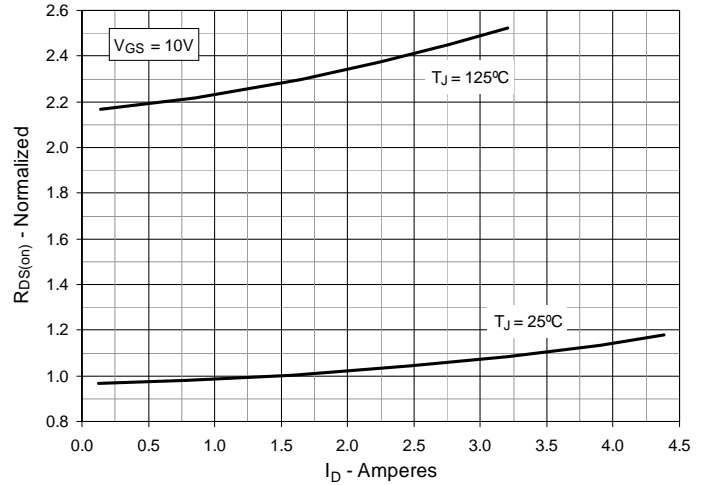
Fig. 4. R_{DS(on)} Normalized to I_D = 1.5A Value vs. Drain Current
