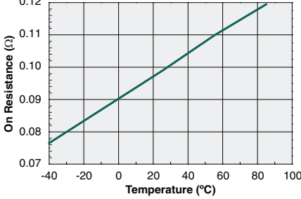
Typical On-Resistance vs. Temperature DC-Only Configuration
