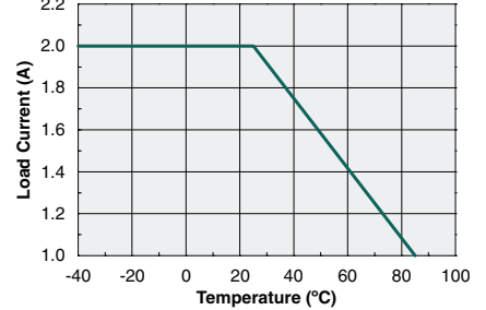
Maximum Load Current vs. Temperature DC-Only Configuration
