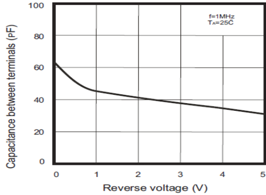
Fig 2 : Junction Capacitance Vs Reverse Voltage Applied
