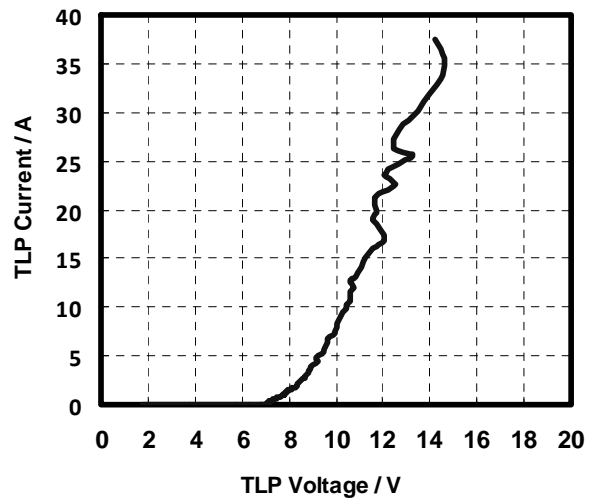
Fig 4 : TLP Measurement
