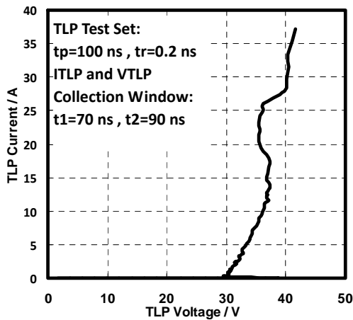
Fig.5 - TLP Measurement
