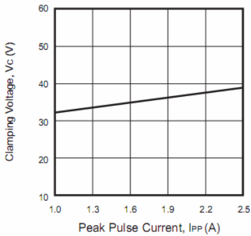
Fig.5 - TLP Measurement
