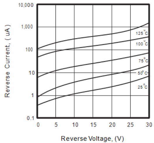
Fig.2 - Reverse Characteristics
