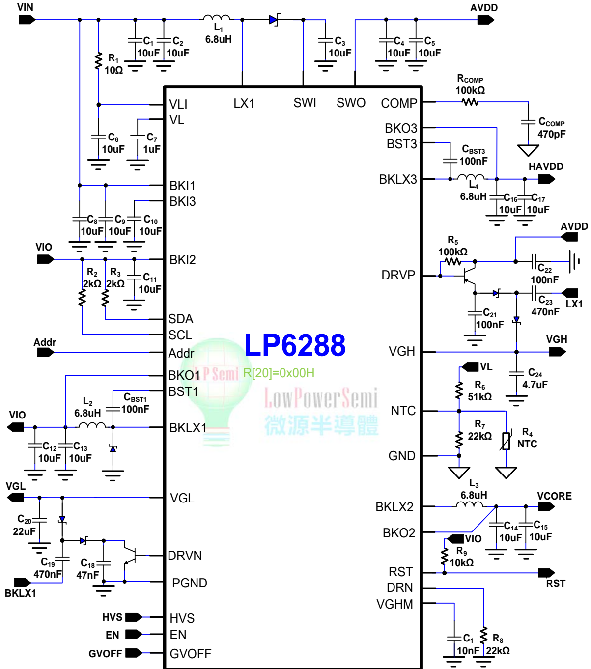
Figure 1. Typical Application Circuit of LP6288 set Internal MOS
