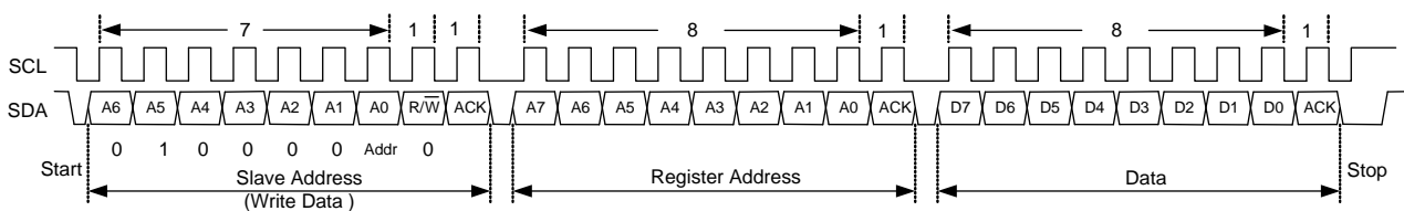
Figure 12. Write Single Byte Data to Register
