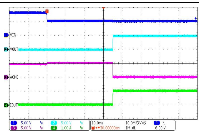
Figure6. OVP Recover @VIN=8V->5V, Load=5Ω
