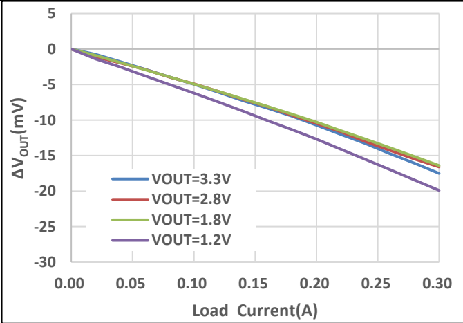
Figure 3. \Delta V_{OUT} vs load current, V_{IN}=V_{OUT}+1V , 25°C
