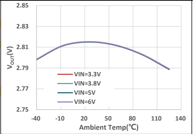
Figure 4. V_{OUT} vs Ambient Temperature, LP3982S-28B5F, I_{OUT}=1mA
