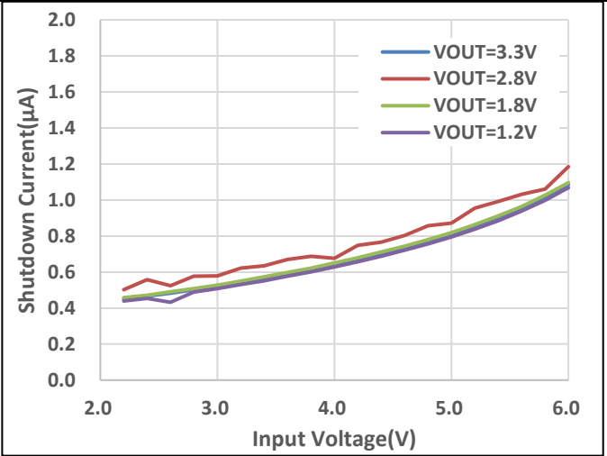
Figure 2. Shutdown current vs input voltage, 25°C
