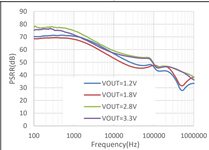
Figure 6. PSRR vs Frequency, I_{OUT}=20mA , V_{IN}=V_{OUT}+1V , 25°C
