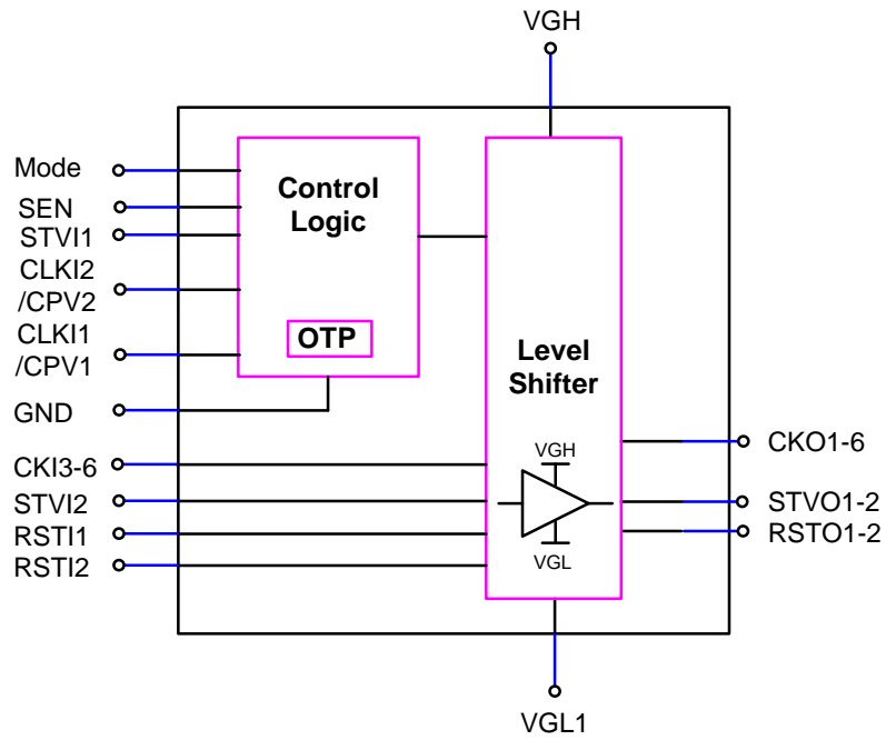
Figure 3. Function Block Diagram
