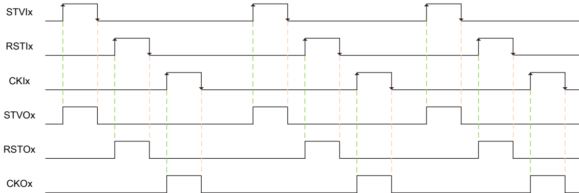
Figure 5. TCON Mode0
