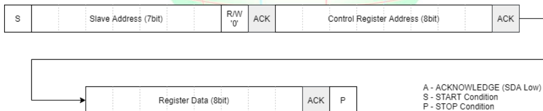
Figure 7. Write Single Byte Data to Register
