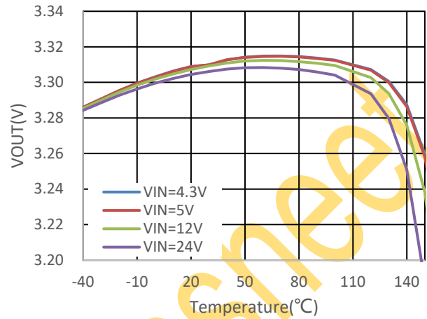
Figure 2. V_{OUT} vs Temperature, LP3994-33B3F, I_{LOAD}=1mA
