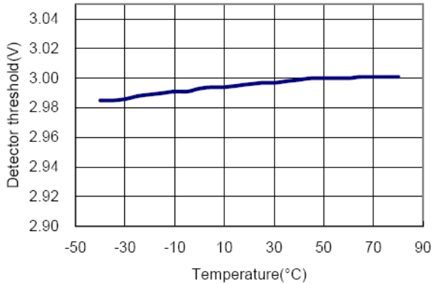
Detector threshold=3.0V
