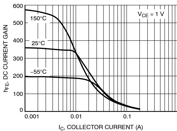
Figure 9. DC Current Gain vs. Collector Current
