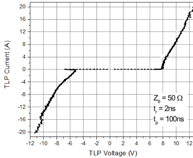
Fig4.TLP Measurement
