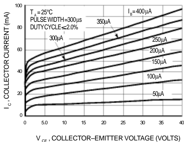
Figure 7. Collector Characteristics
