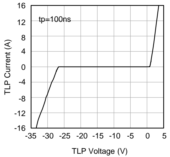
Figure 4. TLP Measurement
