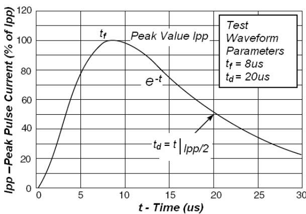
Fig1. Pulse Waveform
