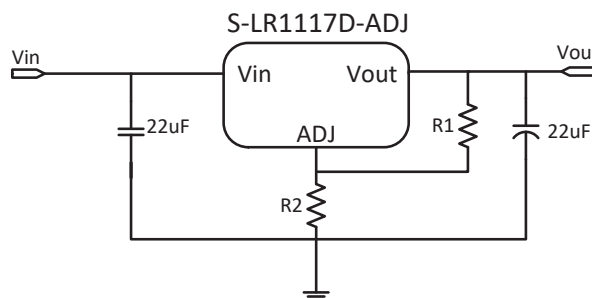
Application Circuit of S-LR1117D-ADJ
