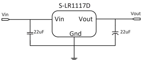
Application circuit of S-LR1117D fixed version
