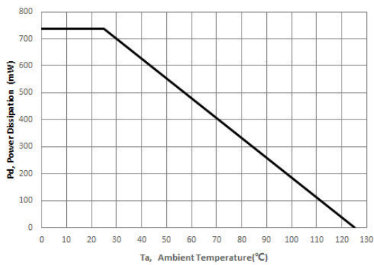
Derating Curve(S-LR117DS)
