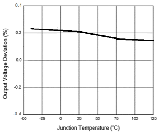
Load Regulation vs. Junction Temperature
