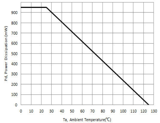
Derating Curve(S-LR117DD)
