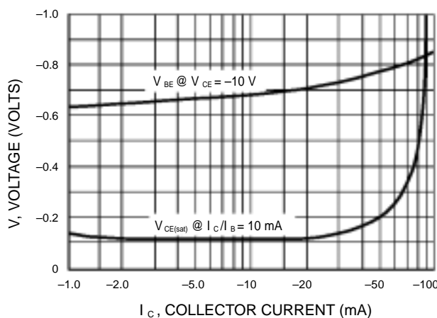
Figure 4. "On" Voltages
