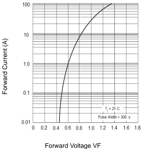
Fig.3 Forward Voltage
