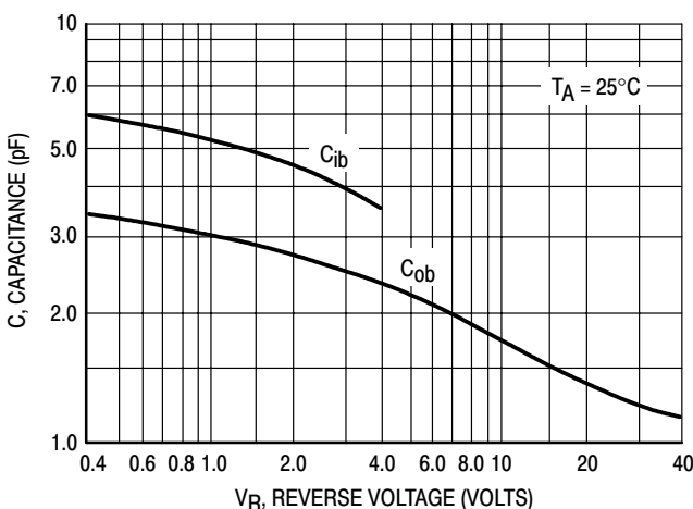
Figure 17. Capacitances
