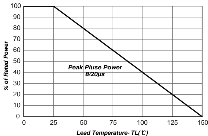
Fig2.Power Derating
