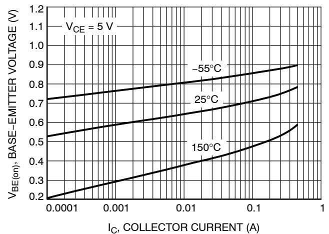
Figure 19. Base Emitter Voltage vs. Collector Current
