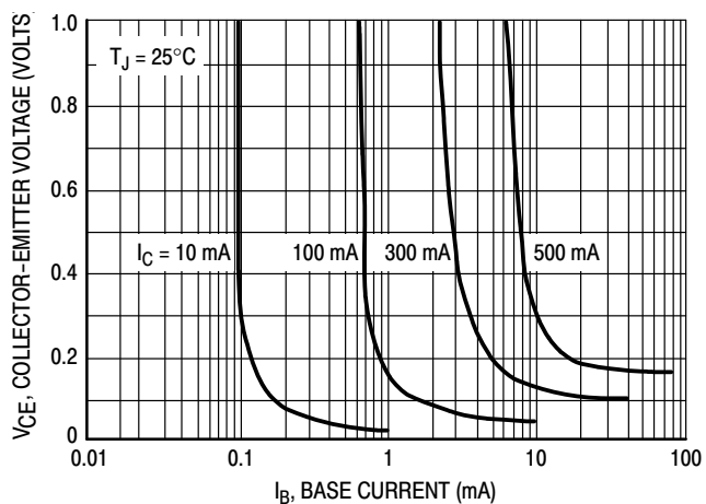
Figure 13. Saturation Region
