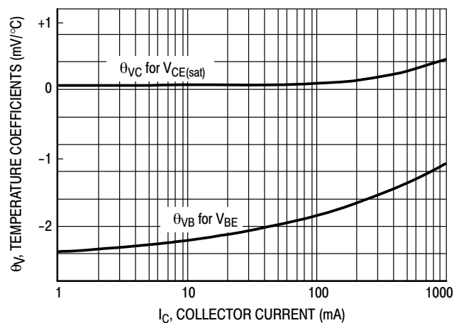
Figure 22. Temperature Coefficients
