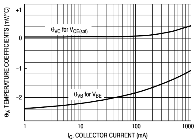
Figure 14. Temperature Coefficients
