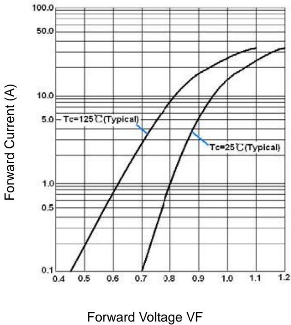
Fig.3 Forward Voltage
