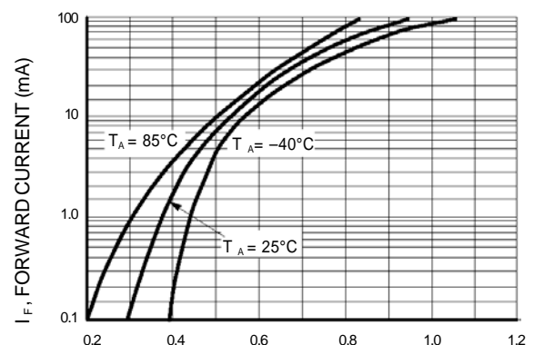
V_F , FORWARD VOLTAGE (VOLTS) Figure 4. Forward Voltage
