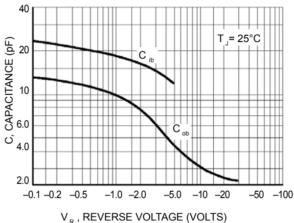
Figure 11. Capacitance
